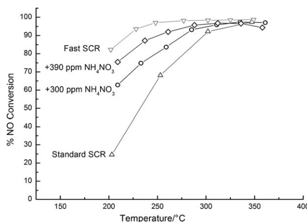
Figure 4. Effect of \text{NH}_4\text{NO}_3 feed concentration on the steady state \text{NO}_x conversion over the \text{V}_2\text{O}_5\text{--WO}_3/\text{TiO}_2 catalyst in comparison to standard and fast SCR. GHSV = 33\,000\text{ h}^{-1} . Feed: 1000 ppm \text{NO}_x , 1000 ppm \text{NH}_3 , 1% \text{H}_2\text{O} , 2% \text{O}_2 in \text{N}_2 . Standard SCR runs: \text{NO}_2/\text{NO}_x = 0 ; fast SCR runs: \text{NO}_2/\text{NO}_x = 1/2 .
